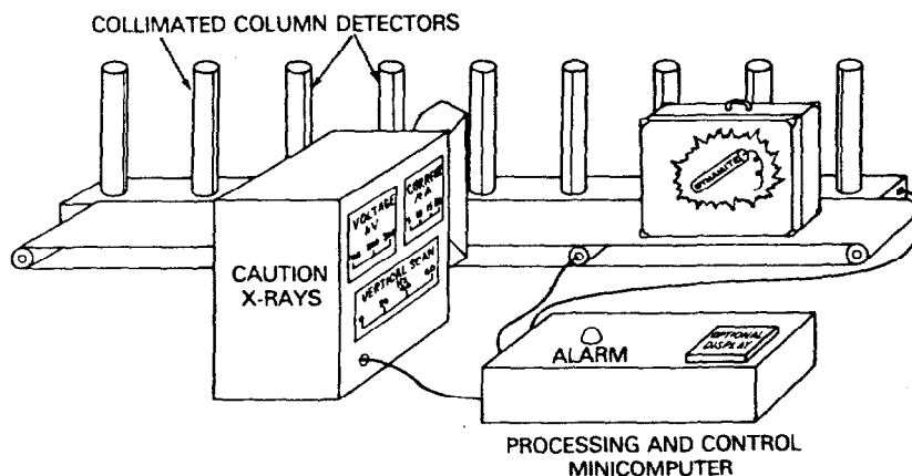
Fig 12 Conceptual Sketch of a CT Explosives Detector
